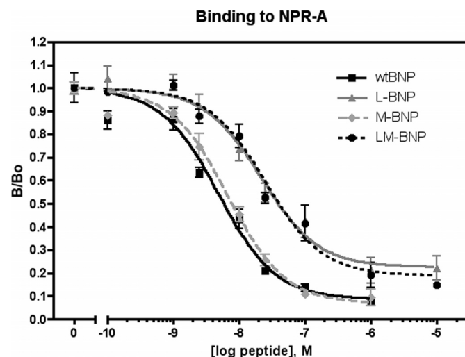
Fig. 4. Mutation of Arg17 to Leu in BNP decreases affinity for human GC-A. 293neo cells stably expressing human GC-A were incubated for 1 h at 4°C with 50 pM ^{125} I-ANP in the presence or absence of increasing concentrations of unlabeled ligand. After washing to remove nonspecific binding, the amount of bound radioligand was quantitated in a gamma counter. The data points represent the mean \pm S.E.M. of three separate experiments assayed in triplicate. wt versus L-BNP, p = 0.028 ; wt versus M-BNP, p = 0.26 ; wt versus LM-BNP, p = 0.042 ; L-BNP versus LM-BNP, p = 0.45 .
