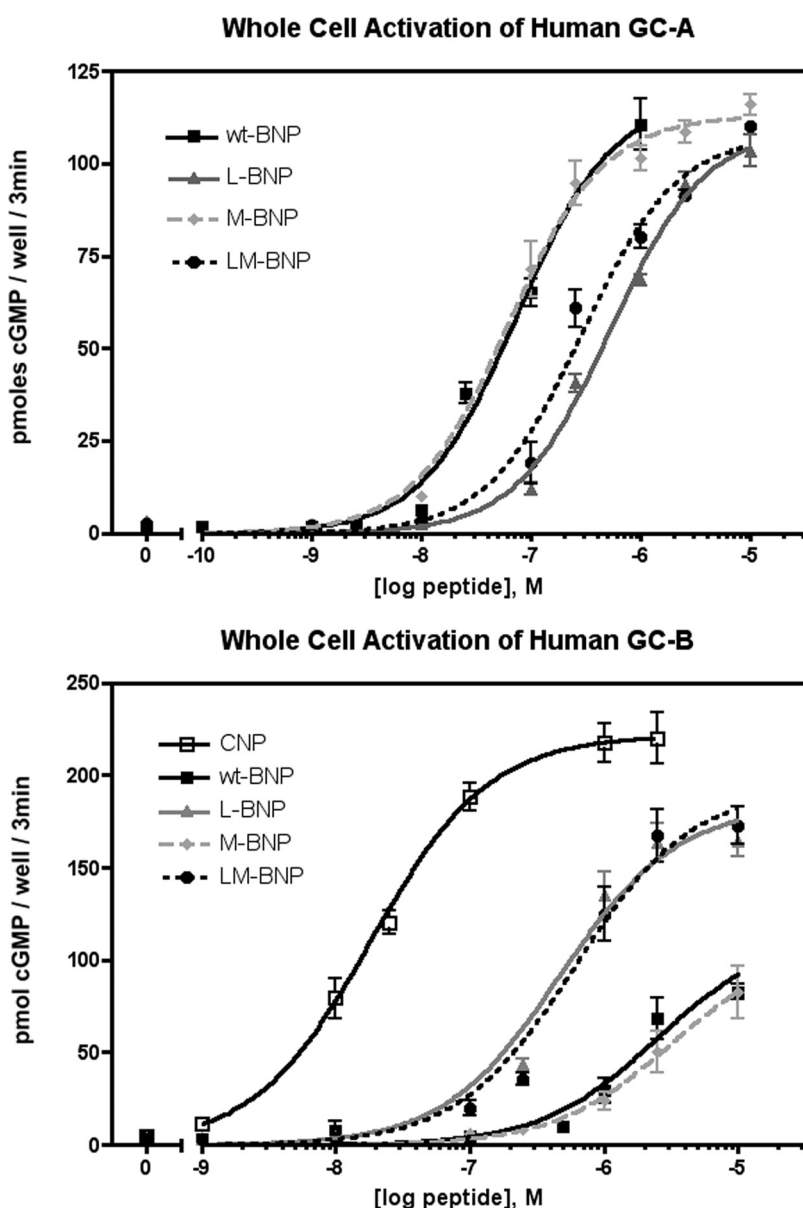
Fig. 2. Mutation of Arg17 to Leu in BNP increases and decreases the EC_{50} for GC-A (top) and GC-B (bottom), respectively. Confluent 293neo cells stably expressing either human GC-A or human GC-B were incubated with increasing concentrations of ligand for 3 min and then cellular cGMP was determined. Top, wt versus L-BNP, p = 0.029 ; wt versus M-BNP, p = 0.69 ; wt versus LM-BNP, p = 0.079 ; L-BNP versus LM-BNP, p = 0.28 . Bottom, wt versus L-BNP, p = 0.085 ; wt versus M-BNP, p = 0.19 ; wt versus LM-BNP, p = 0.07 ; L-BNP versus LM-BNP, p = 0.0008 .
