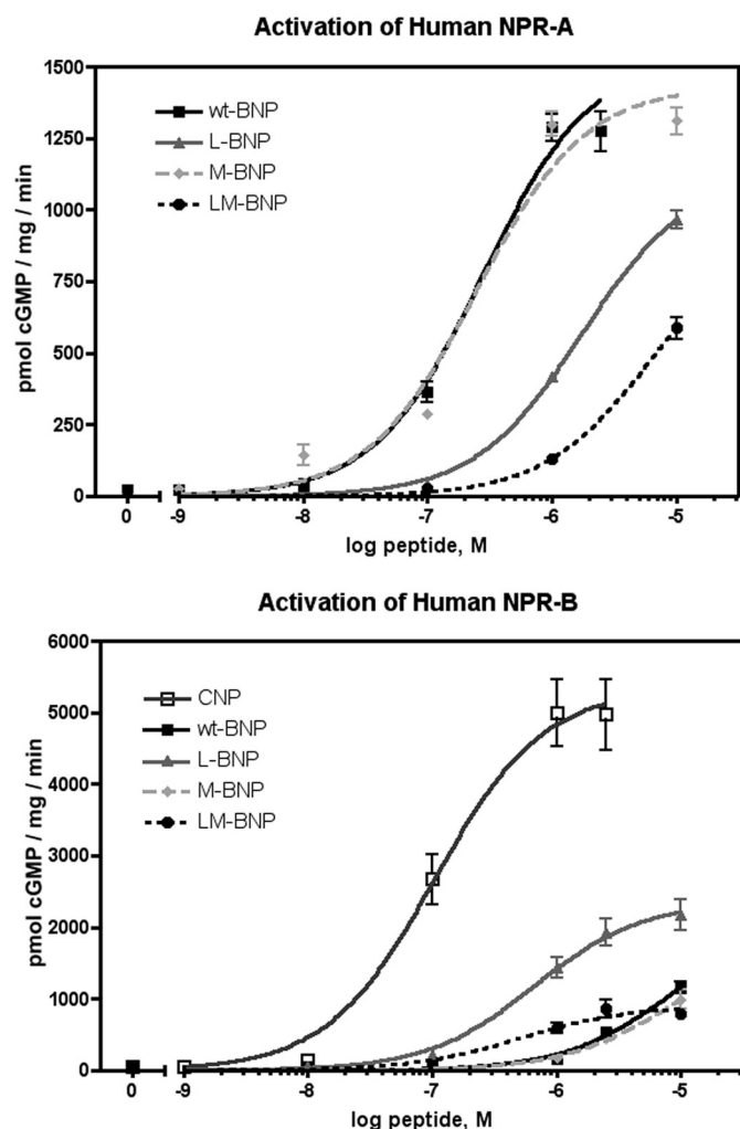
Fig. 3. Mutation of Arg17 to Leu in BNP increases and decreases the EC_{50} for GC-A and GC-B activity, respectively. Crude membranes from 293neo cells stably expressing human GC-A (top) or human GC-B (bottom) were incubated for 3 min at 37°C in the presence or absence of increasing concentrations of various BNP-derived peptides. Guanylyl cyclase activities were determined and plotted as a function of BNP concentrations.
