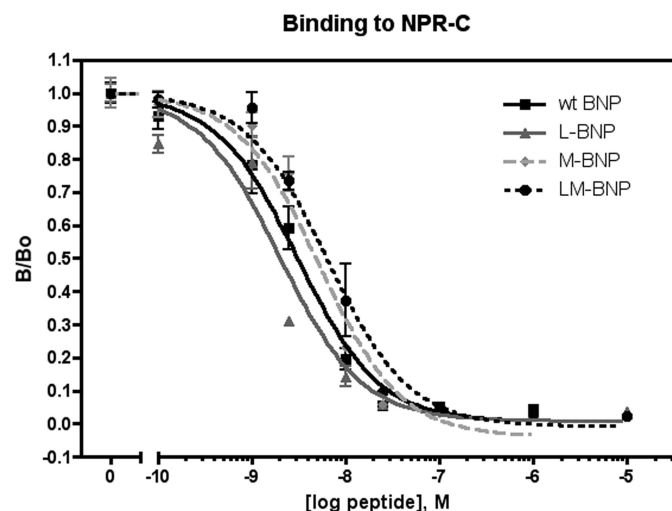
Fig. 5. Wild-type BNP and L-BNP bind NPR-C with similar affinities. 293neo cells stably expressing human NPR-C were incubated with ^{125}I -ANP in the presence or absence of increasing concentrations of unlabeled ligand as described above. The amount of specific binding is shown. The data points represent the mean \pm S.E.M. of two separate experiments assayed in triplicate. wt versus L-BNP, p = 0.058 ; wt versus M-BNP, p = 0.016 ; wt versus LM-BNP, p = 0.002 ; L-BNP versus LM-BNP, p < 0.0001 .
